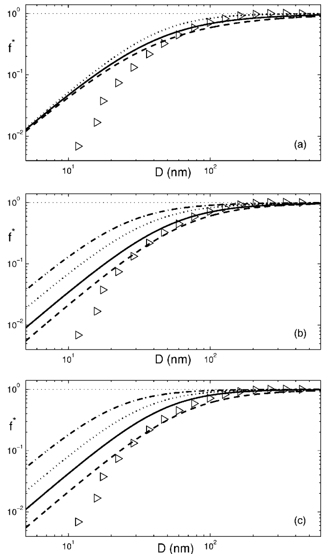
FIG. 3. A comparison between the experiment from Ref. [8] with d=1.6 nm and \omega=10 Hz ( \triangleright ) and the model for different bubble sizes, contact angles, and surface coverage. (a) Influence of bubble size; model with surface coverage \phi=0.99 , contact angle \theta=150^\circ , and bubble sizes R_0=1 nm (dotted line), 25 nm (solid line), and 50 nm (dashed line). (b) Influence of contact angle; model with surface coverage \phi=0.99 , bubble size R_0=10 nm, and contact angles \theta=120^\circ (dashed line), 140^\circ (solid line), 160^\circ (dotted line), and 170^\circ (dashed-dotted line). (c) Influence of surface coverage; model with bubble size R_0=10 nm, contact angle \theta=120^\circ , and surface coverage \phi=0.1 (dashed-dotted line), \phi=0.25 (dotted line), \phi=0.5 (solid line), and \phi=0.99 (dashed line).
