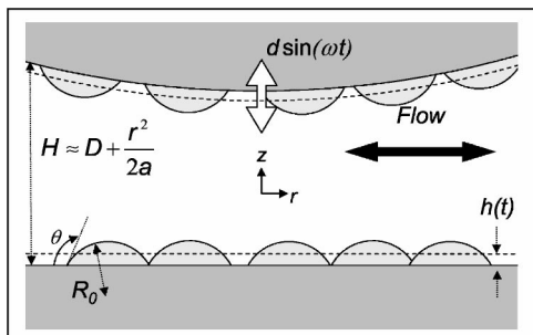
FIG. 1. A typical squeeze flow experiment: a solid sphere of radius a is oscillated in a liquid at a distance D \ll a of a smooth solid surface with amplitude d \ll D and frequency \omega . The surfaces are covered by microscopic gas bubbles of contact angle \theta and radius of curvature R_0 . The set of bubbles is approximated by a gas layer of time evolving thickness h(t) .
