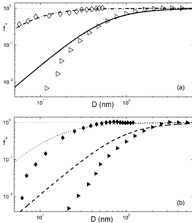
FIG. 2. A comparison between the experimental data of Zhu and Granick (2001) and the dynamic model (23) with R_0=10 nm and \phi=99\% . (a) Small amplitude experimental data; ( \diamond ): measurements for d=0.5 nm, \omega=1 Hz; dashed-dotted line: model for \theta=177^\circ ; ( \triangleright ): measurements for d=1.6 nm, \omega=10 Hz; solid line: model for \theta=132^\circ . (b) Large amplitude experimental data. ( \diamond ): measurements for d=6 nm, \omega=1 Hz; dotted line: model for \theta=168^\circ ; ( \triangleright ): measurements for d=6 nm, \omega=10 Hz; dashed line: model for \theta=90^\circ .
